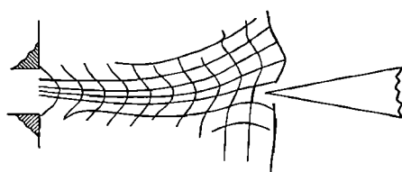
FIG. 2. Streamlines and velocity profiles during edge tone oscillation from Shields. 10
