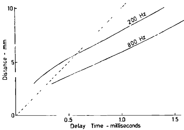
FIG. 5. Propagation of centerline crossing for two different exciting frequencies. Jet centerline initial velocity 1000 cm/sec. Dashed line uniform propagation at 1000 cm/sec.
