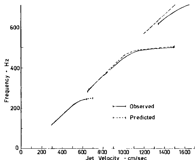
FIG. 10. Observed and predicted frequencies of oscillation for a low- Q organ pipe.
