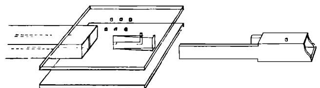
FIG. 6. Sketch of enclosed jet edge system, and the removable pipe that could be fitted in to make an organ pipe.
