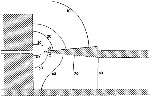
FIG. 8. Contours of acoustic pressure (relative peak values) for the organ pipe sounding in its first mode at 250 Hz.
