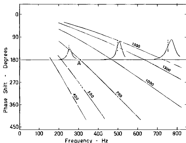
FIG. 4. Phase shifts on the jet (long lines labeled with centerline velocities in cm/sec) and in the organ pipe (humped curves). The passive resonance frequencies of the three pipe modes are at the vertical dashed lines. Slit to edge distance 7 mm.
