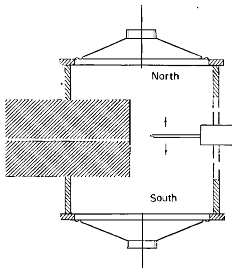
FIG. 3. Cross section of arrangement of slit blocks, loud-speaker exciter and Pitot tube microphone for measuring jet phase.
