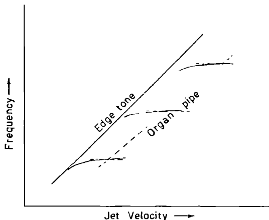
FIG. 1. Frequency behavior of jet-edge oscillators.
