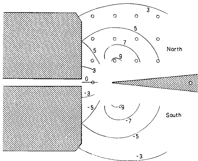
FIG. 7. Contours of acoustic pressure (relative peak values) during edge tone generation. Frequency 419 Hz, slit-to-edge distance 7 mm.
