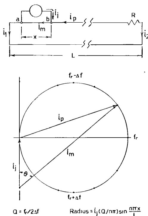
FIG. 9. Equivalent circuit for organ pipe and jet current drive, with vector diagram showing current relationships in the neighborhood of a pipe resonance.
